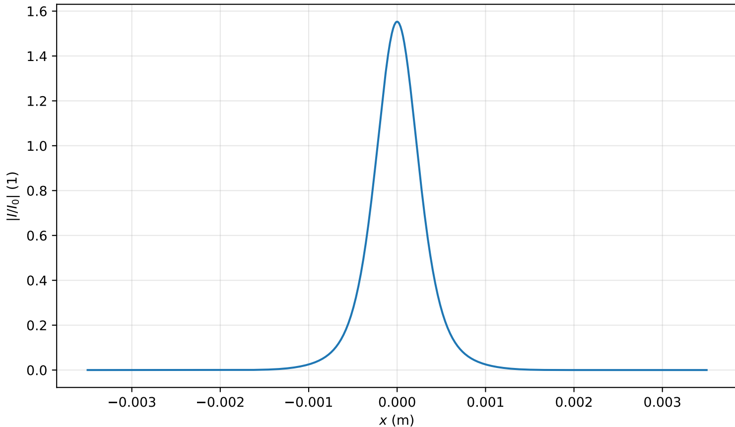
Intensity profile I(x, y = 0, z = 1.433m)/I_0 , P_{in}=0.9P_{cr} , artificial time
